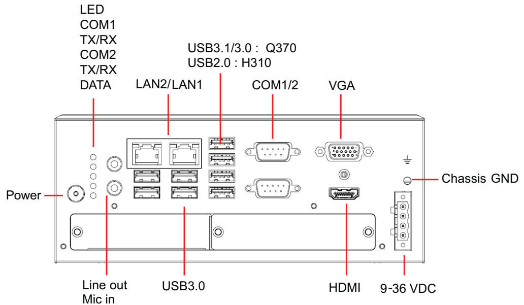
Figure 2.1 MIC-770 Front View
